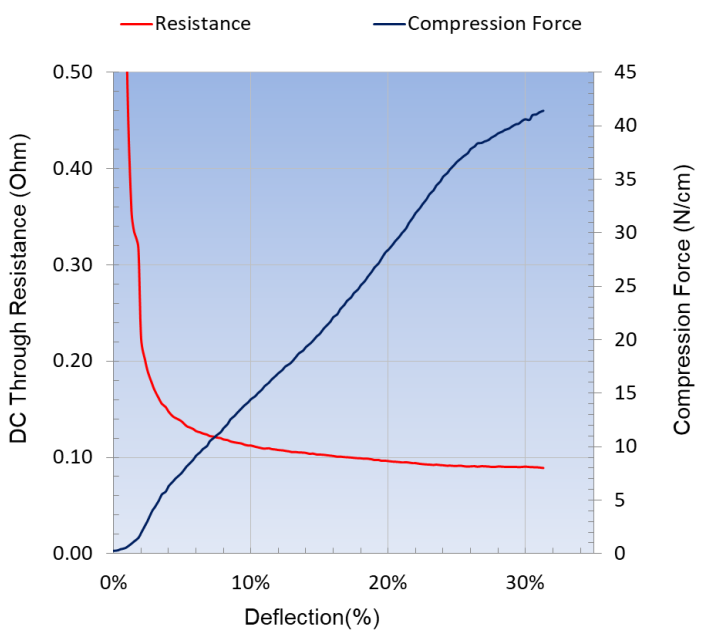
Force-Deflection-Resistance Curve of F5321 Gasket 1.00mm (H) X 1.30mm (W) X 5.00mm (L)
