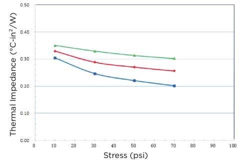
Thermal Impedance Vs. Stress of GP8100-H1/H0/HU (1.0mm thick) (at Temp=60°C; Step application of pressure 10, 30, 50, 70 psi; ASTM D5470 modified)
