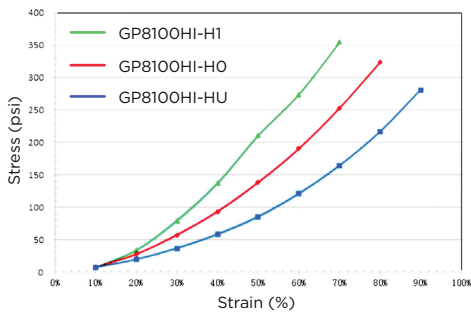
Stress Vs. Strain of GP8100HI-HI/HO/HU (1.0mm thick) with Constant Rate of Strain (@ Temp=25-29°C; Constant Rate of Strain = 0.01 inch/min)
