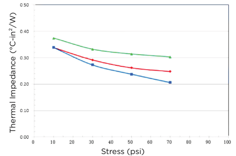
Thermal Impedance Vs. Stress of GP8100HI-HI/HO/HU (1.0mm thick) (at Temp=60°C; Step application of pressure 10, 30, 50, 70 psi; ASTM D5470 modified)
