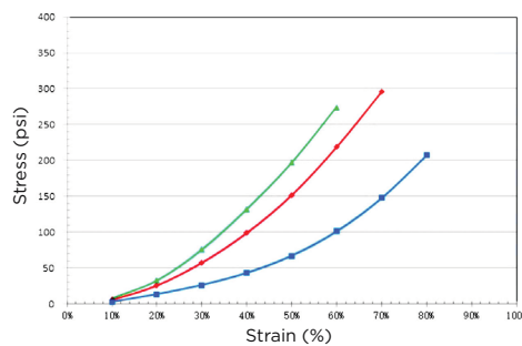
Stress Vs. Strain of GP8100HI-HI/HO/HU (1.0mm thick) with Step Application of Strain (@ Temp=25-29°C; Rate of Strain = 0.01 inch/min between each step application of strain; stress measurement time interval of 2 min for each step application of strain)
