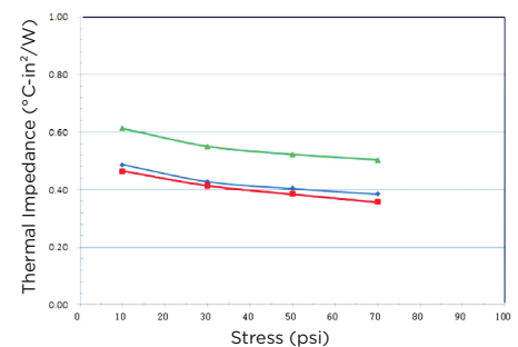
Thermal Impedance Vs. Stress of GP5100-H1/H0/HU (1.0mm thick) (at Temp=60°C; Step application of pressure 10, 30, 50, 70 psi; ASTM D5470 modified)
