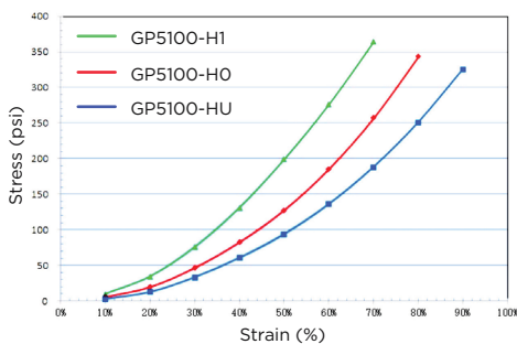
Stress Vs. Strain of GP5100-H1/H0/HU (1.0mm thick) with Constant Rate of Strain (@ Temp=25-29°C; Constant Rate of Strain = 0.01 inch/min)
