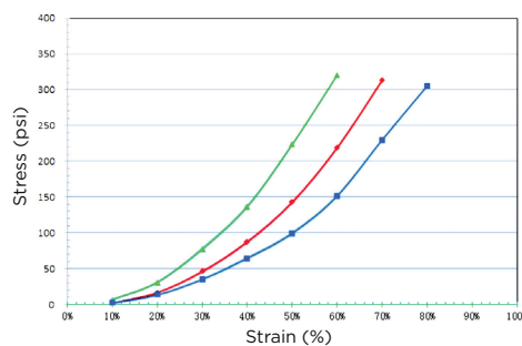
Stress Vs. Strain of GP5100-H1/H0/HU (1.0mm thick) with Step Application of Strain (@ Temp=25-29°C; Rate of Strain = 0.01 inch/min between each step application of strain; stress measurement time interval of 2 min for each step application of strain)
