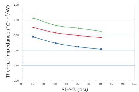
Thermal Impedance Vs. Stress of GP3100-H1/H0/HU (1.0mm thick) (at Temp=60°C; Step application of pressure 10, 30, 50, 70 psi; ASTM D5470 modified)
