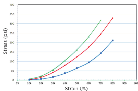
Stress Vs. Strain of GP3100-H1/H0/HU (1.0mm thick) with Step Application of Strain (@ Temp=25-29°C; Rate of Strain = 0.01 inch/min between each step application of strain; stress measurement time interval of 2 min for each step application of strain)
