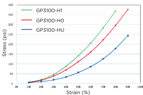
Stress Vs. Strain of GP3100-H1/H0/HU (1.0mm thick) with Constant Rate of Strain (@ Temp=25-29°C; Constant Rate of Strain = 0.01 inch/min)
